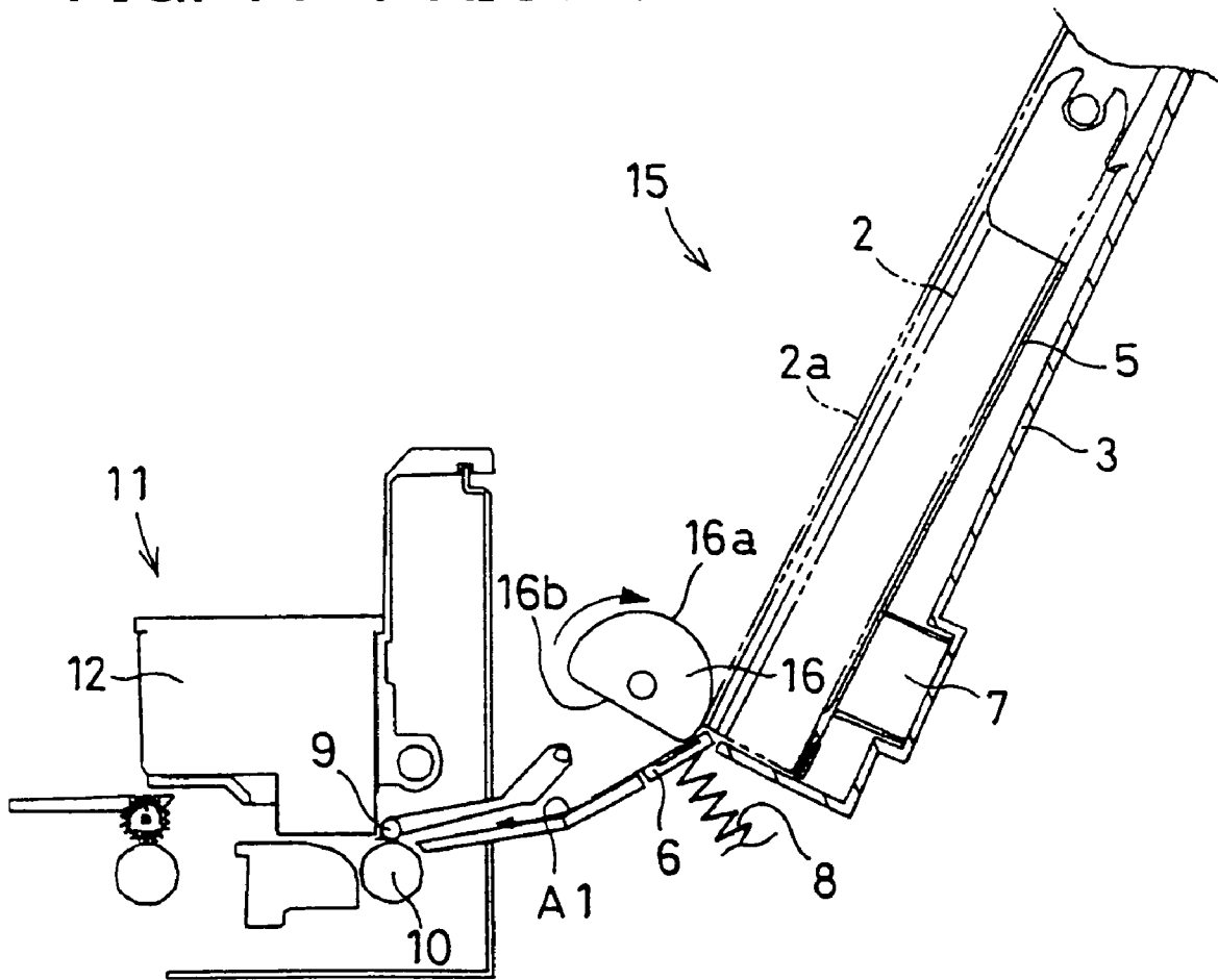
FIG. 11 PRIOR ART
