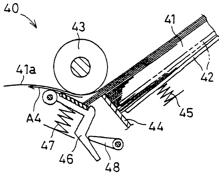
FIG. 14 PRIOR ART
