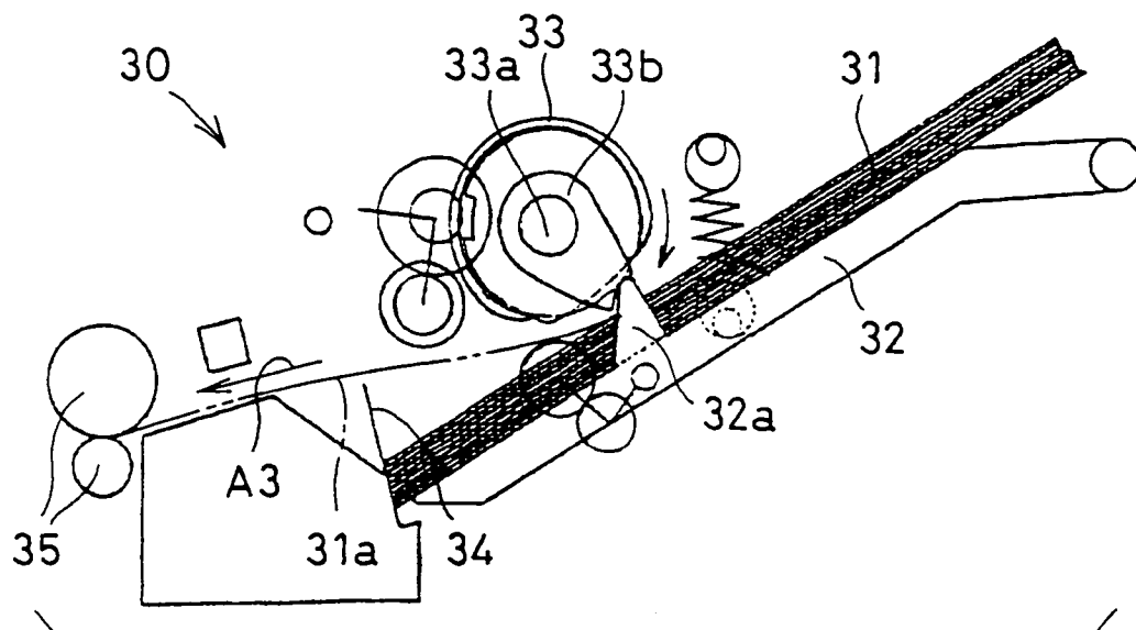
FIG. 13 PRIOR ART
