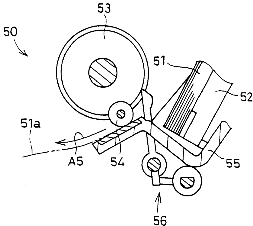
FIG. 15 PRIOR ART
